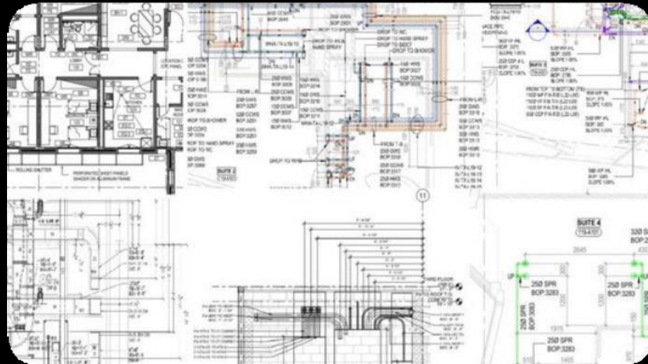
SHOP DRAWINGS
